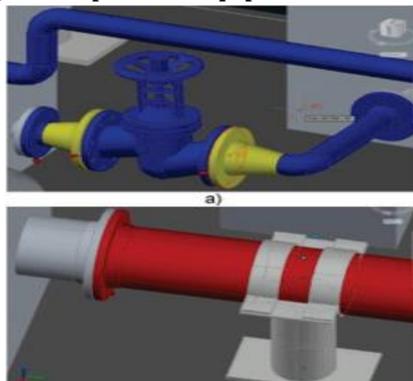
Figure 6 Block valve DN100 and steam line arm DN250
