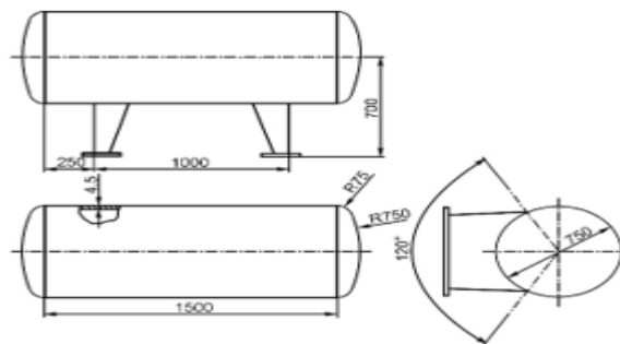
Figure 4 Tank dimensions
