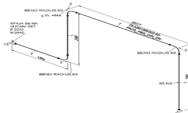
Figure 10 Part of pipeline modeled in Revit
