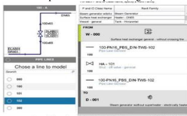
Figure 8 Status information and modification of pipeline model DLAB01BR003
