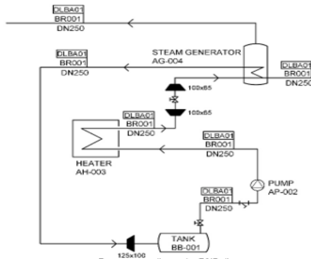
Figure 2 Process according to the P&ID diagram
